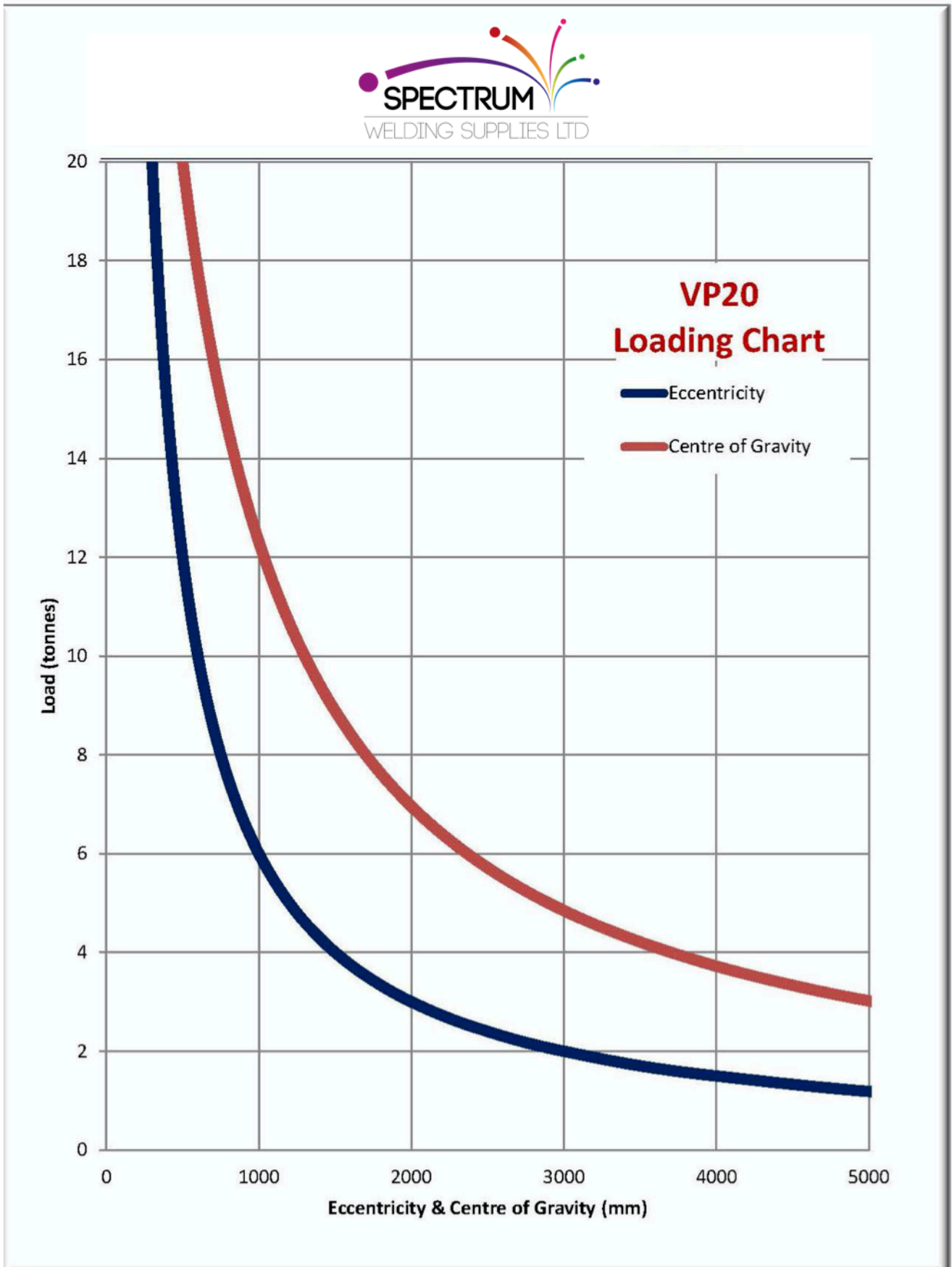
Figure 2 Loading Chart
