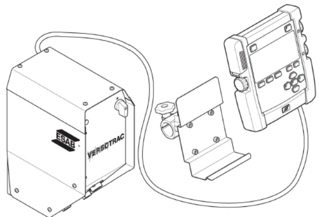
EAC 10 controller with motor drive unit, mounting bracket and control cable included
